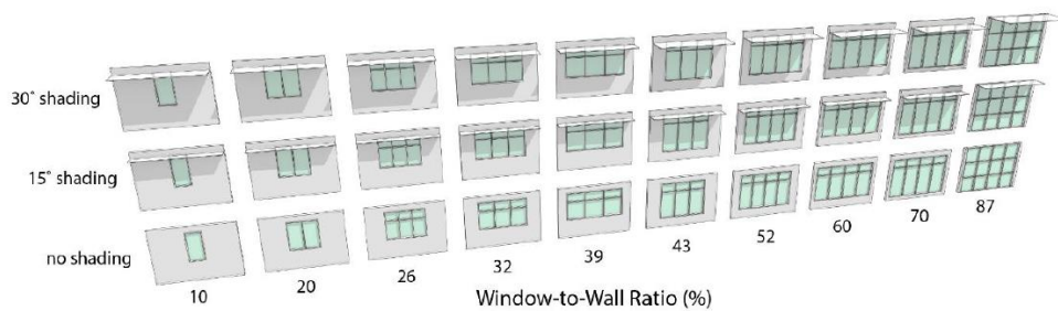
Figure 2-3 –Window-to-wall ratio (WWR) is the percentage of glazing areas relative to its exterior wall envelope areas. (Code of Environmental Sustainability of Buildings)
