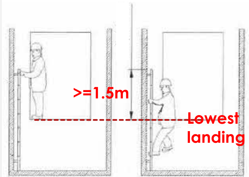
Type 1 - Fixed pit ladder
