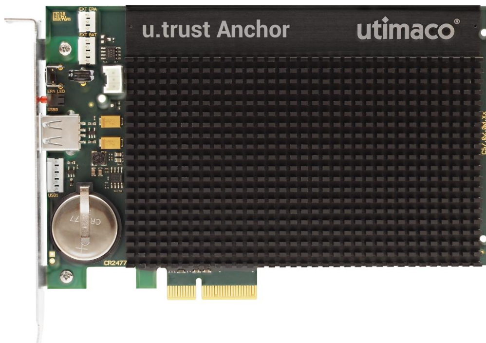
Figure 1: u.trust Anchor
