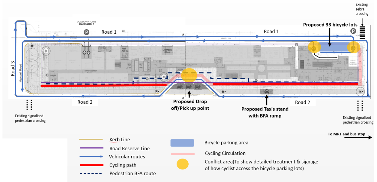
Figure B.2a – Example of a Circulation Plan
