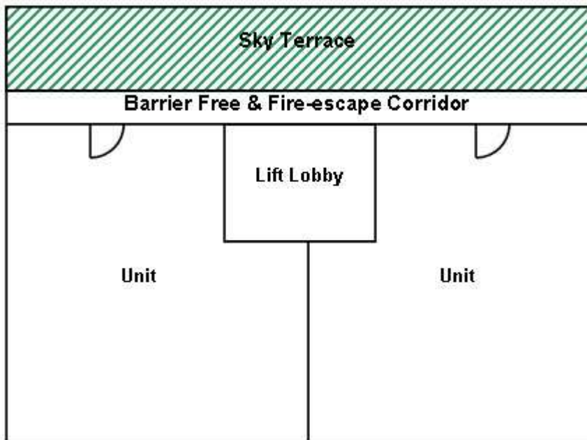
Figure B: Sky terrace occupying less than 60% of floor plate Corridor is to be computed as GFA.
