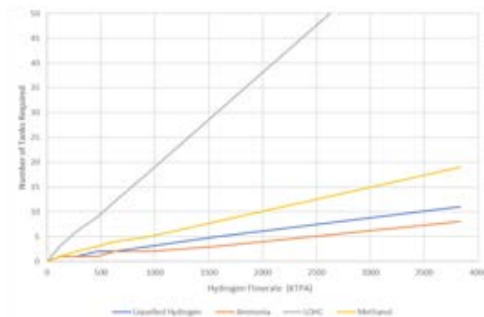
Figure 5.12 – Number of Storage Tanks Required in Singapore per carrier vs Increasing Hydrogen Volumes
