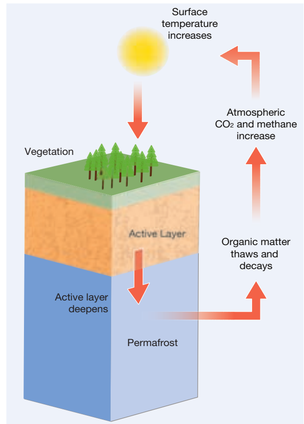
Figure 21: The permafrost carbon feedback is an amplification of surface warming due to the thaw of organic material currently frozen in permafrost, which will then decay and release CO 2 and methane into the atmosphere.
