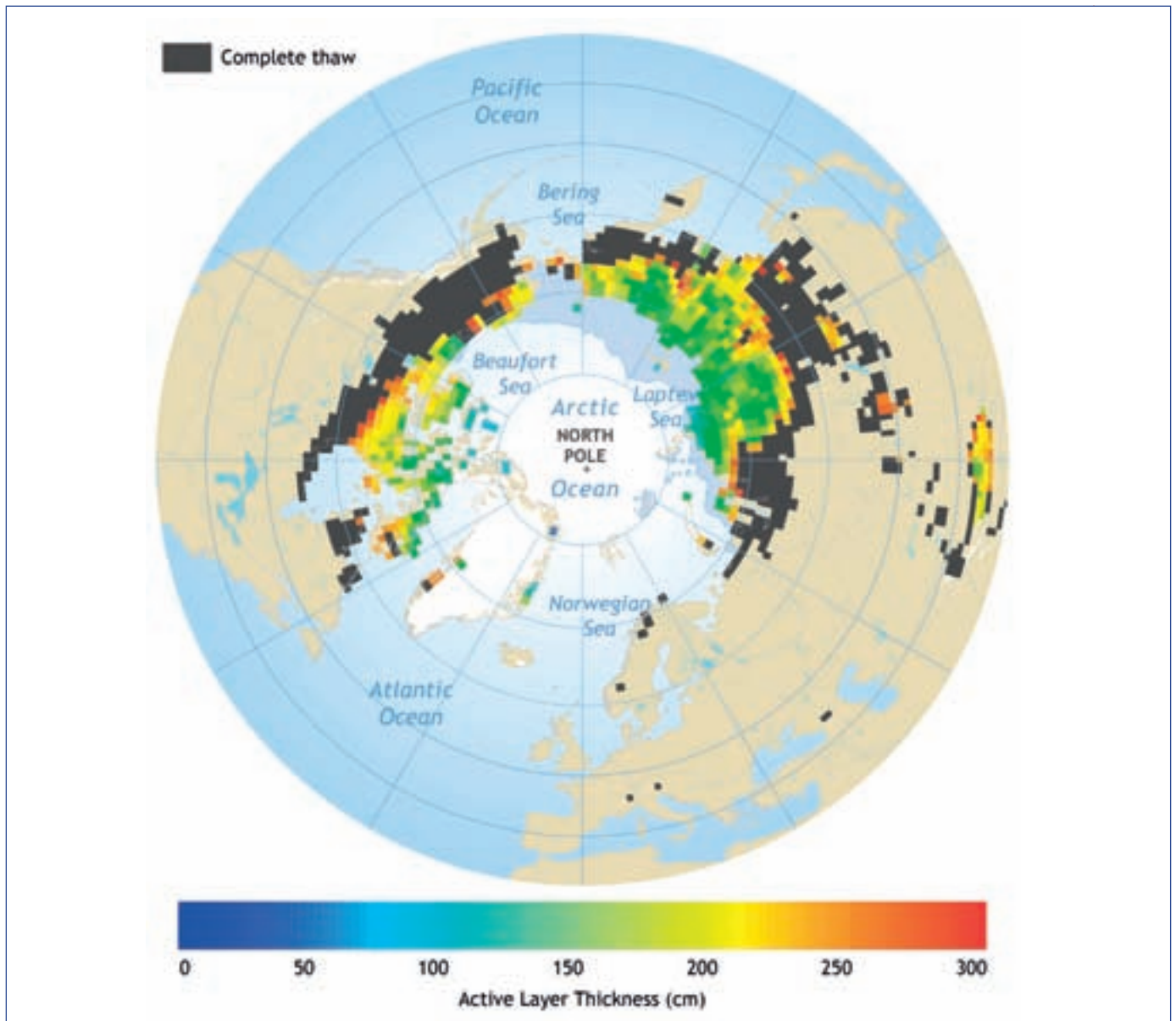
Figure 12: This model projection indicates a 59% loss in near-surface permafrost area by 2100 for the IPCC A1B scenario. The dark grey regions show where taliks may form and permafrost in the top 1.5 meters of soil may completely thaw (Schaefer et al. 2011).
